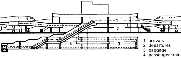
7 Section through satellite → 6
